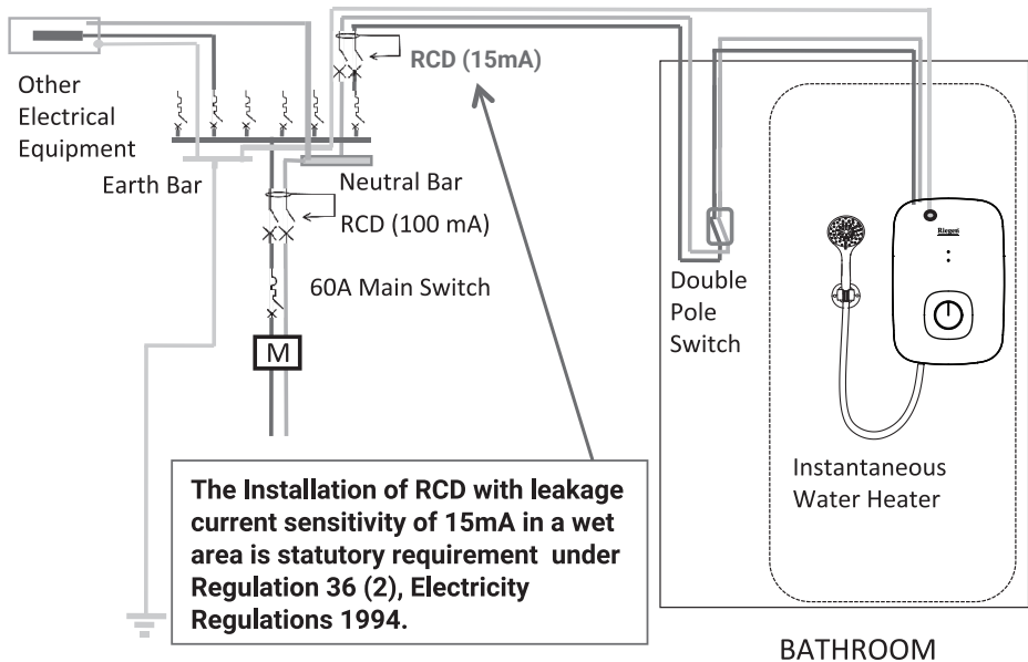
Figure 7: The installation of RCD for instantaneous water heater with leakage current sensitivity of 15mA in a wet area.
